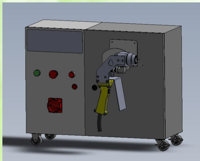
The CiQ-6001 Low Capacity Flame Treatment Unit Paired with Cirqual®iQ
